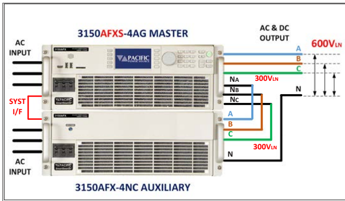
30kVA Series Output Configuration
