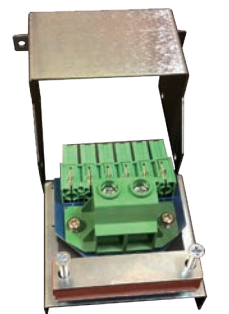
Single Phase Mode Output Adaptor Option
